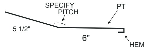
TRANSITION TRIM
