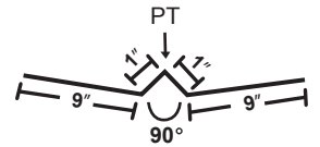
VALLEY FLASHING
