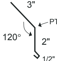
EAVE TRIM
